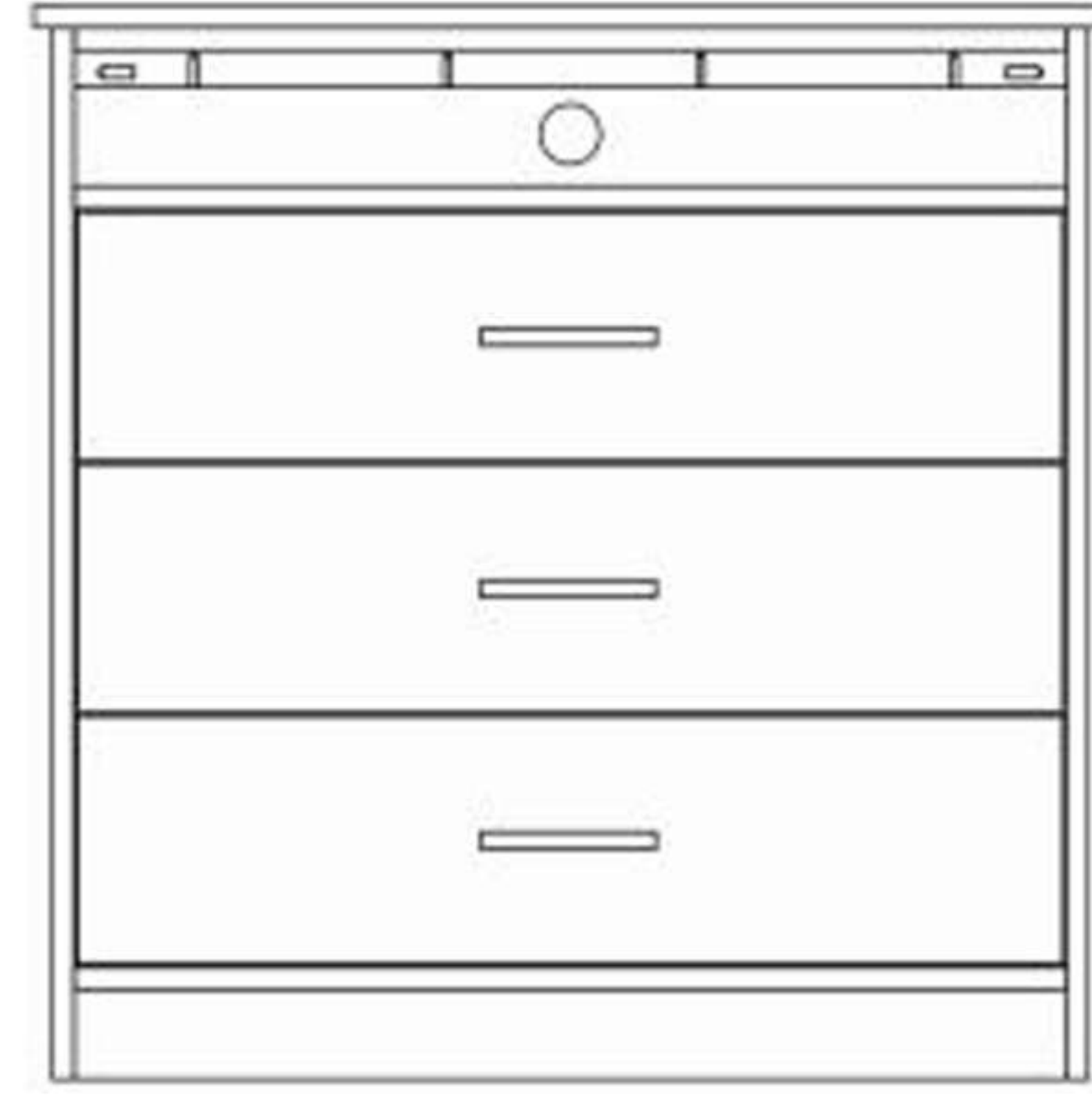
Three Drawer Chest w/ Shelf 36"wx22"dx36"h
