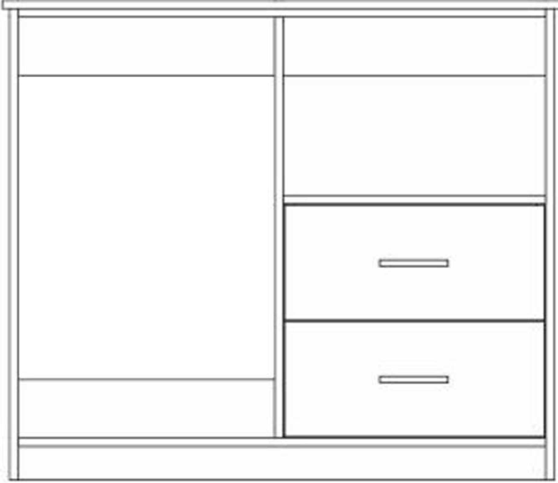
Microfridge 48"wx22"dx43"h
